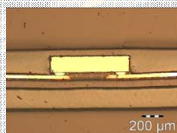
Encapsulated RFID chip
